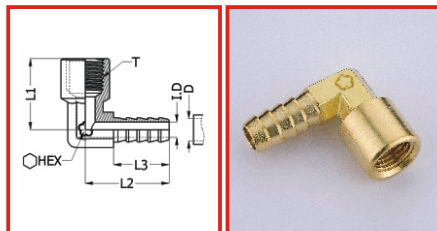
內牙插心彎頭 Female Hose-Barb Elbow
