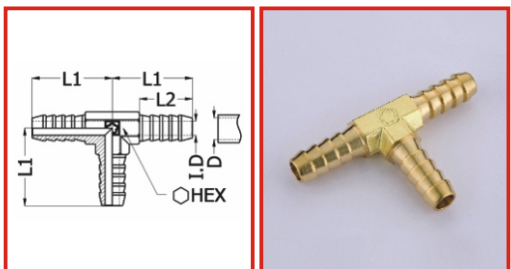
插心三通 Union Hose-Barb Tee
