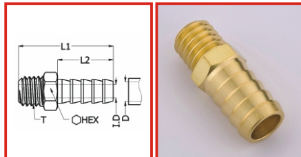
惠氏牙插心接頭 Whitworth male Hose-Barb Connector
