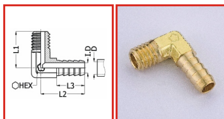
惠氏牙插心彎頭 Whitworth male Hose-Barb Elbow
